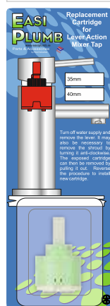
Replacement 40mm Monobloc Cartridge Type 3
