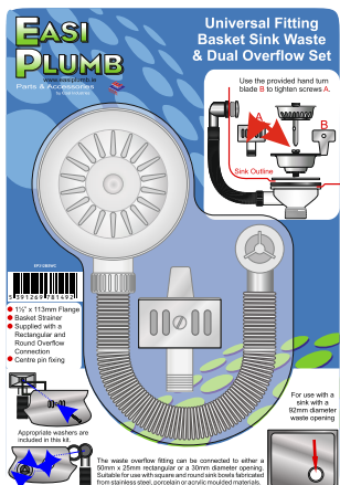
3 1/2" Basket Strainer Sink Waste with Round & Rectangular Overflow Components
