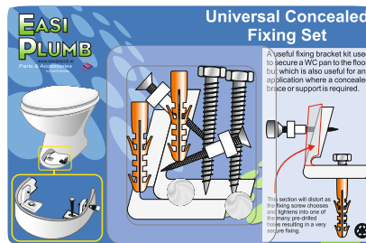
Universal Concealed Fixing Set
