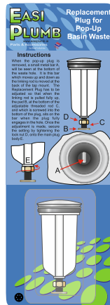
Replacement Plug for Pop Up Waste
