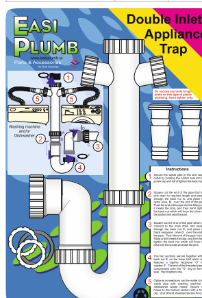
Double Inlet Appliance Trap
