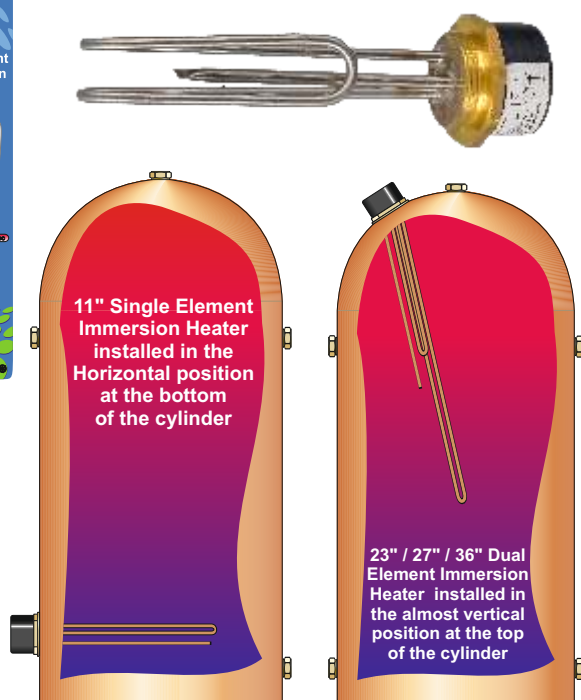
Single Element Incoloy Immersion Heater
