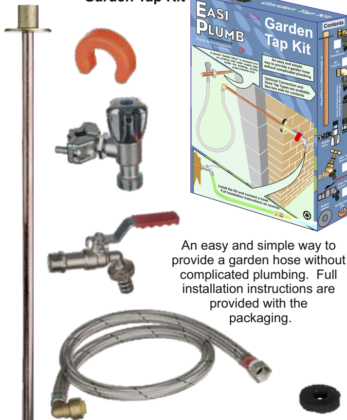
Garden Tap Kit
