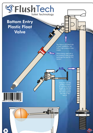
Bottom Entry Plastic Float Valve
