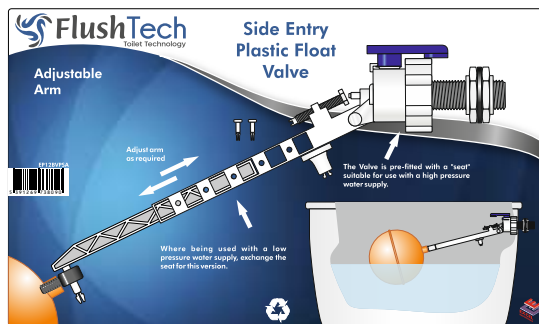
Side Entry Plastic Float Valve
