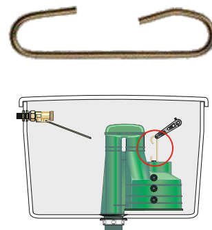
"C" Link Siphon Lift Arm Connector
